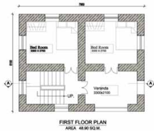
TWO-STOREY+TERRACE
