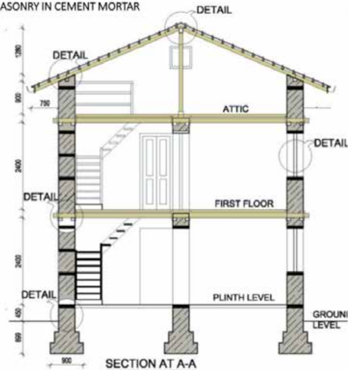
Model SMC-2.5: STONE MASONRY IN CEMENT MORTAR
